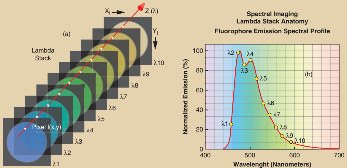
FIG. 16 A 3D spectral image cube. There are two dimensions to the cube ( x, y ) from the image itself and a third one from the measured wavelength. (Illustration by G. H. Bearman.)
